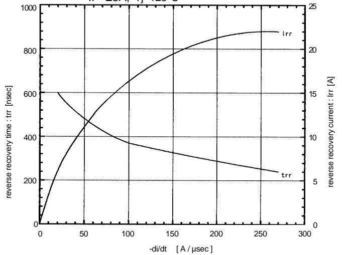
Reverse recovery time characteristics vs. -di/dt IF=25A, Tj=125°C
