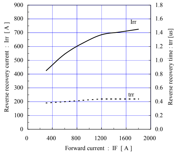
Reverse recovery characteristics (typ.) Vce=600V, VGE=±15V, Rgon=2Ω, Tj=125°C
