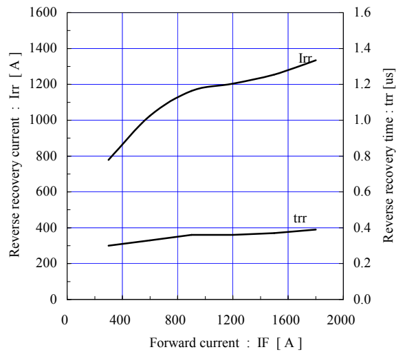
Reverse recovery characteristics (typ.) Vcc=900V, VGE=±15V, Rgon=3.9Ω, Tj=125°C
