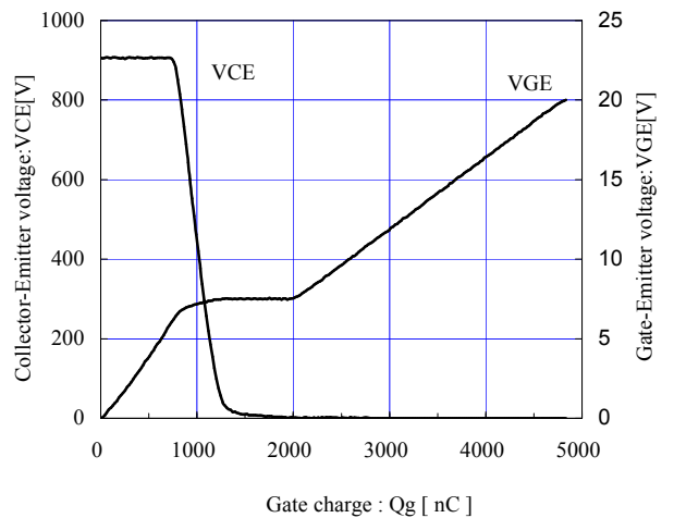
Dynamic Gate charge (typ.) Tj= 25°C
