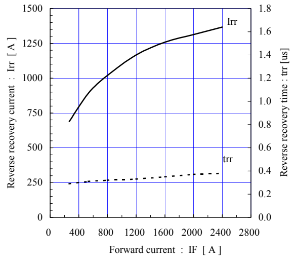
Reverse recovery characteristics (typ.) Vcc=600V, VGE=±15V, Rgon=1.5Ω, Tj=125°C
