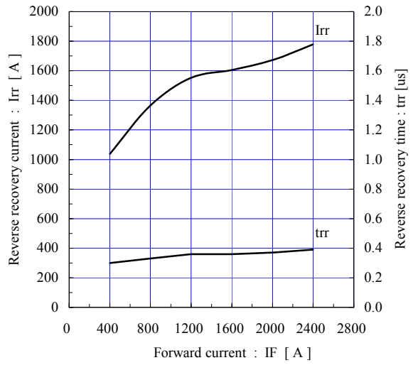
Reverse recovery characteristics (typ.) Vcc=900V, VGE=±15V, Rgon=2.7Ω, Tj=125°C
