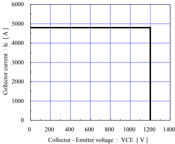
Reverse bias safe operating area (max.) \pm V_{GE}=15V, T_i=125^\circ C / \text{chin}
