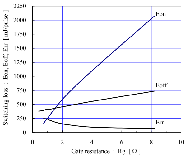
Switching loss vs. Gate resistance (typ.) V_{cc}=600V, I_c=2400A, V_{GE}=\pm 15V, T_j=125^\circ C
