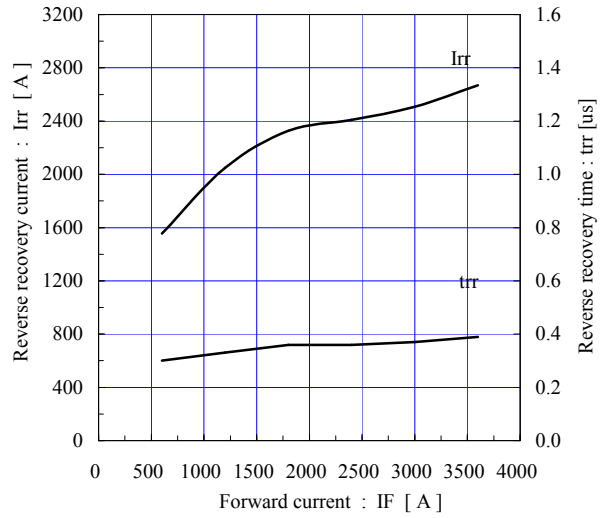
Reverse recovery characteristics (typ.) Vcc=900V, VGE=±15V, Rgon=1.8Ω, Tj=125°C
