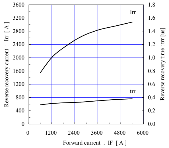
Reverse recovery characteristics (typ.) Vcc=600V, VGE=±15V, Rgon=0.6Ω, Tj=125°C
