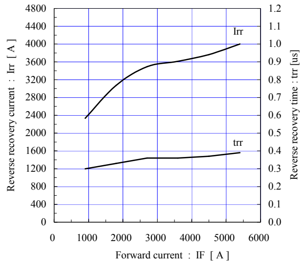
Reverse recovery characteristics (typ.) Vcc=900V, VGE=±15V, Rgon=1Ω, Tj=125°C
