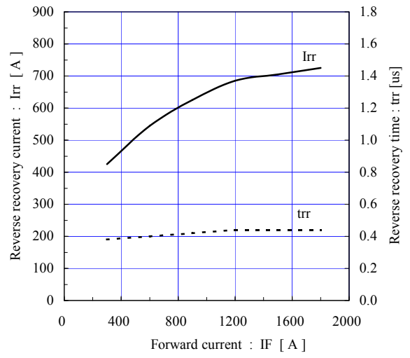
Reverse recovery characteristics (typ.) Vcc=600V, VGE=±15V, Rgon=3.3Ω, Tj=125°C
