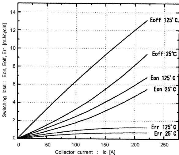
Switching loss vs. Collector current Vcc=300V, RG=16 ohm, VGE=±15V
