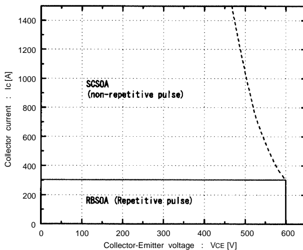
Reversed biased safe operating area +VGE=15V, -VGE ≤ 15V, Tj ≤ 125°C, RG ≥ 16 ohm
