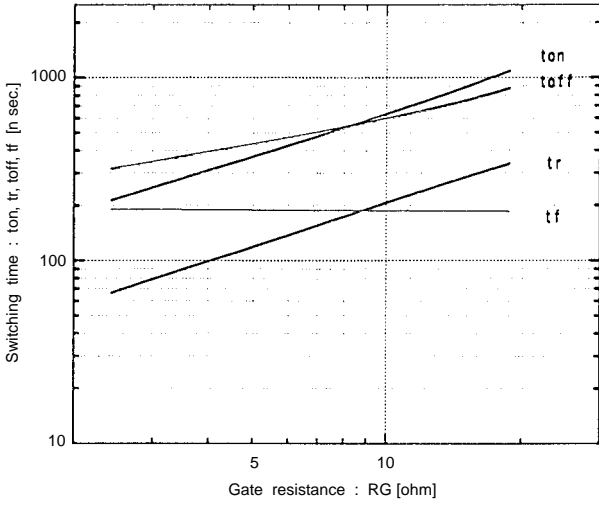
Switching time vs. RG Vcc=300V, Ic=200A, VGE=±15V, Tj=25°C
