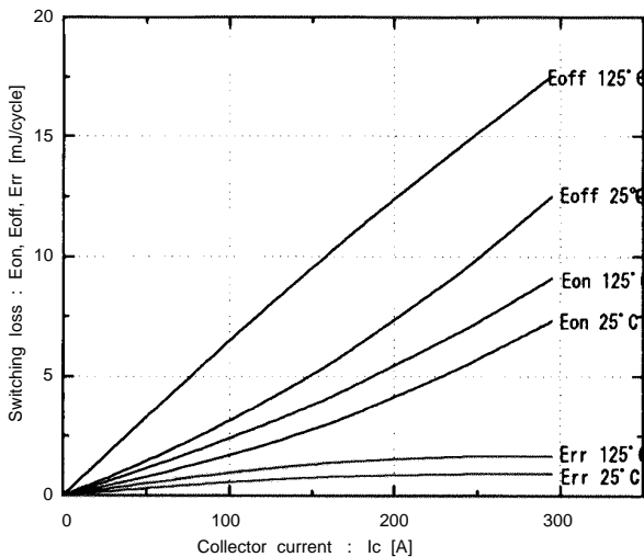
Switching loss vs. Collector current Vcc=300V, RG=9.1 ohm, VGE=±15V
