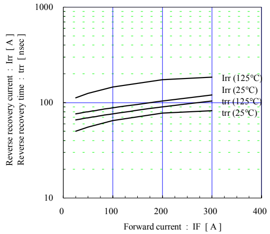
Reverse recovery characteristics (typ.) V cc =300V, V GE =±15V, R g =16Ω
