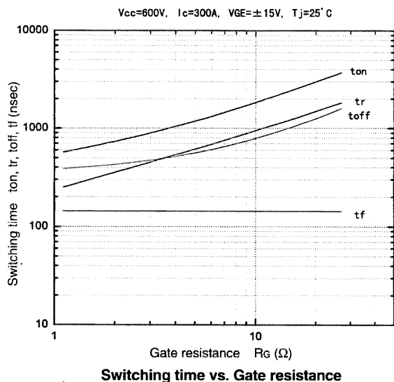
Switching time vs. Gate resistance
