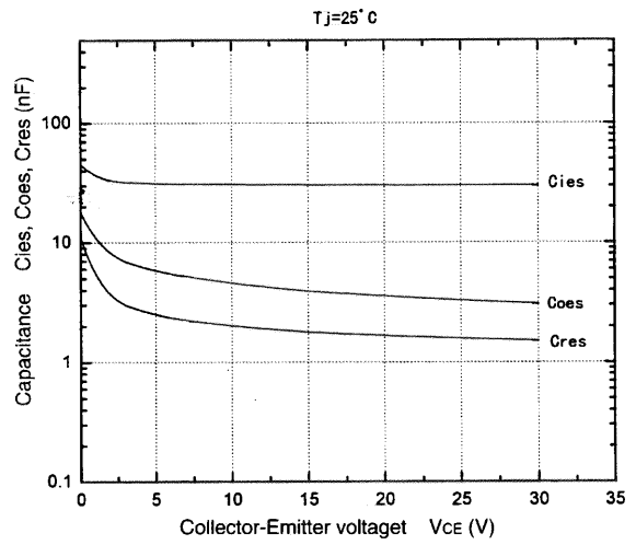
Capacitance vs. Collector-Emittet voltage
