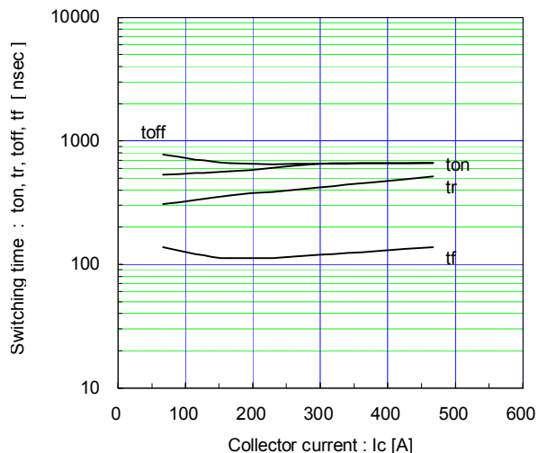
Switching time vs. Collector current (typ.) V_{cc}=900V, V_{GE}=\pm 15V, R_g=1.5\Omega, T_j=125^\circ C
