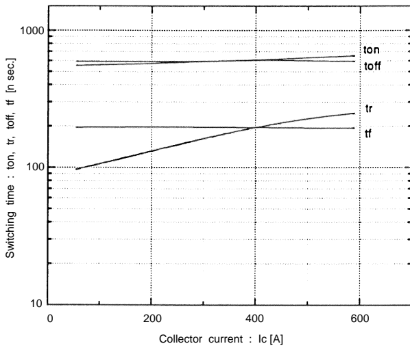
Switching time vs. Collector current V CC =300V, R G =4.7 ohm, V GE =±15V, T J =25°C
