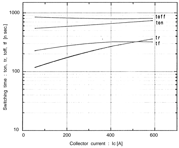
Switching time vs. Collector current V CC =300V, R G =4.7 ohm, V GE =±15V, T J =125°C
