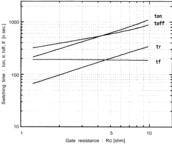
Switching time vs. RG Vcc=300V, Ic=400A, VGE=±15V, Tj=25°C
