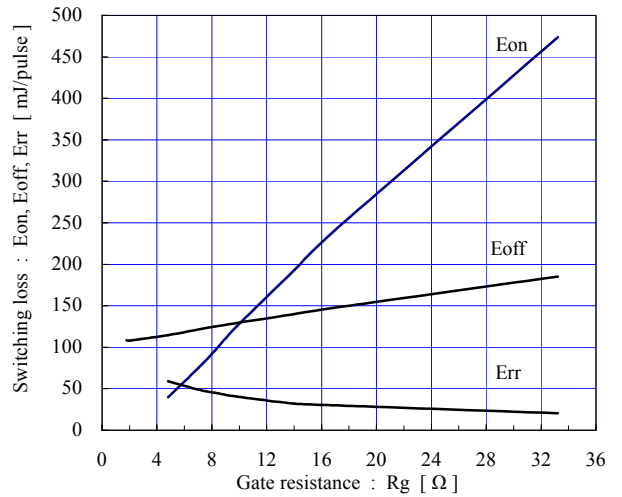
Switching loss vs. Gate resistance (typ.) V_{cc}=600V, I_c=600A, V_{GE}=\pm 15V, T_j=125^\circ C
