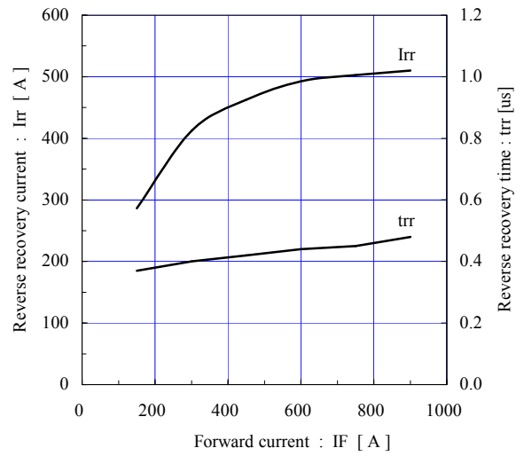
Reverse recovery characteristics (typ.) Vcc=900V, VGE=±15V, Rg=12Ω, Tj=125°C
