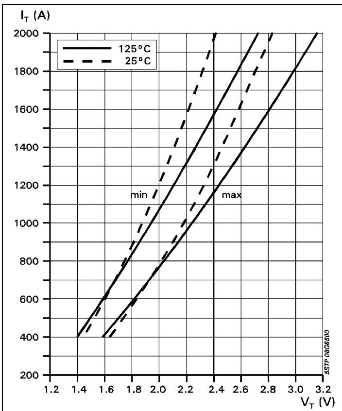
Fig 2. On-state characteristics.
