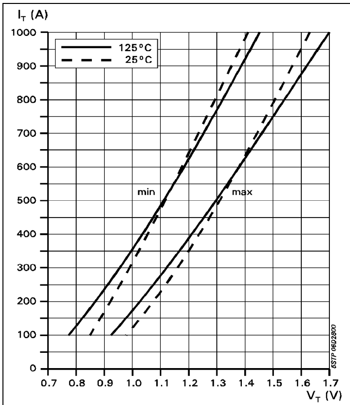
Fig. 2. On-state characteristics.
