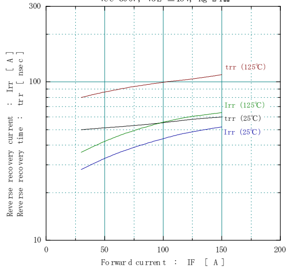
[ Inverter ] Reverse recovery characteristics (typ.) Vc=300V, VGE=±15V, Rg=24Ω
