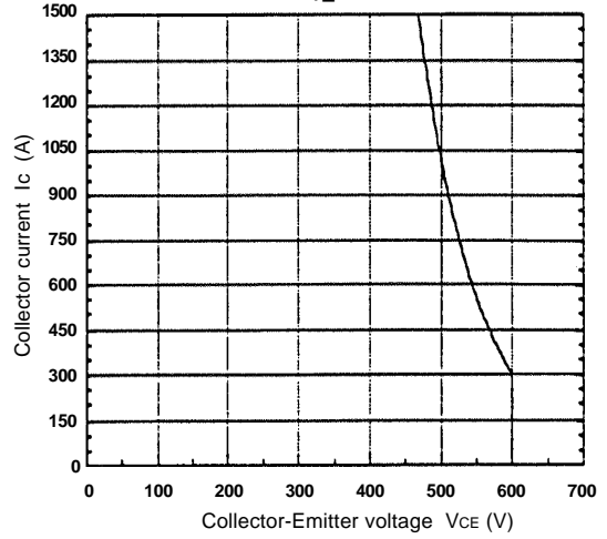
Reverse biased safe operating area Vcc=15V, Tj≤125°C
