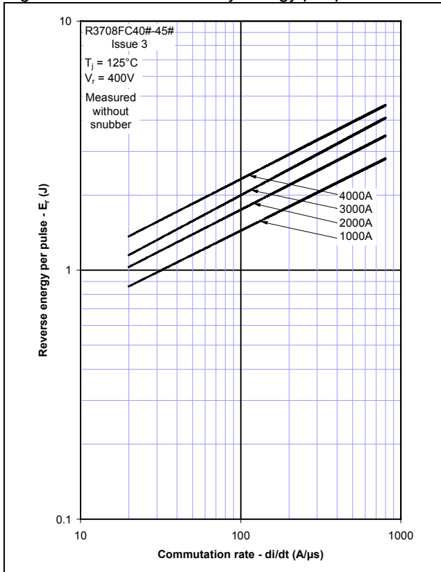
Figure 9 – Reverse recovery energy per pulse
