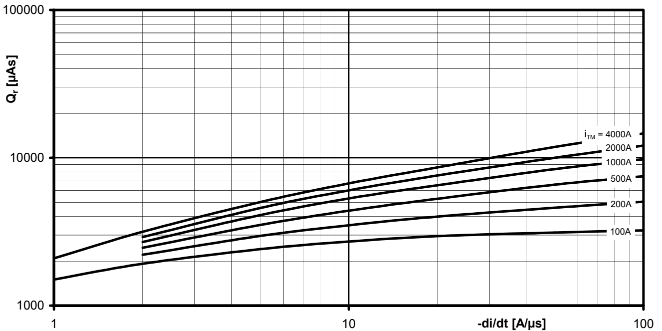
Sperrverzögerungsladung / Recovered charge Q_r = f(di/dt)
