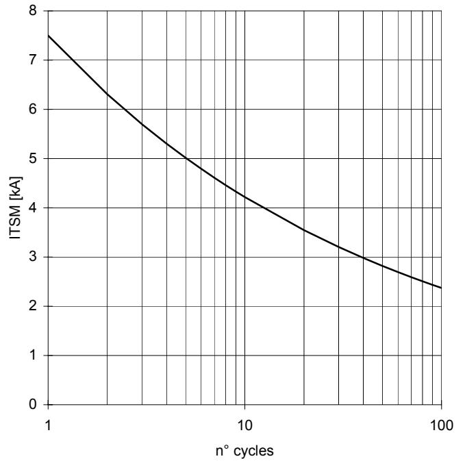
SURGE CHARACTERISTIC T_j = 125\text{ }^\circ\text{C}
