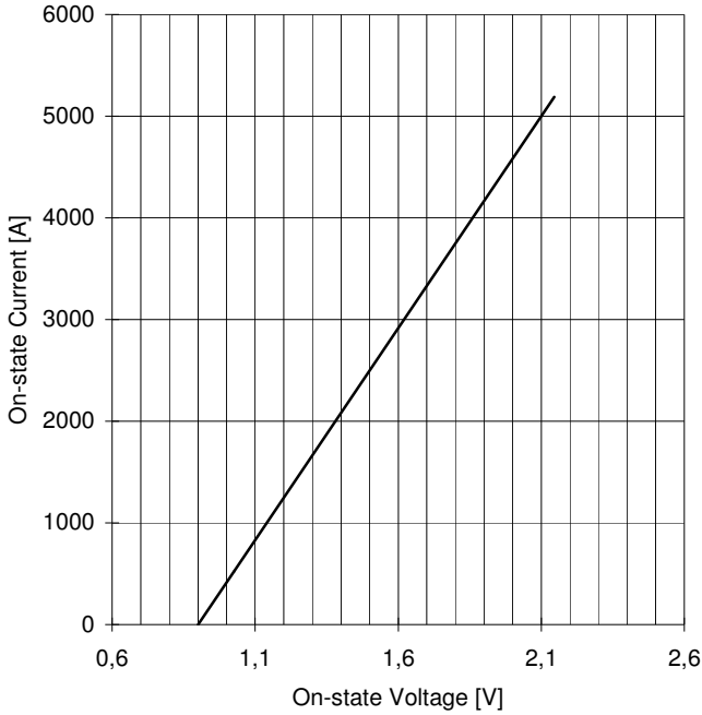
ON-STATE CHARACTERISTIC T_j = 125\text{ }^\circ\text{C}
