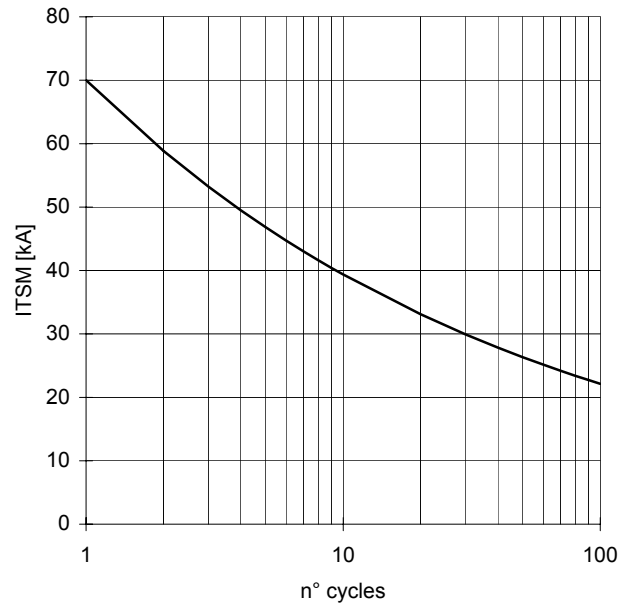
SURGE CHARACTERISTIC T_j = 140\text{ }^\circ\text{C}
