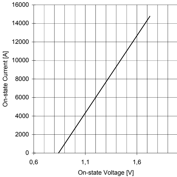
ON-STATE CHARACTERISTIC T_j = 140\text{ }^\circ\text{C}
