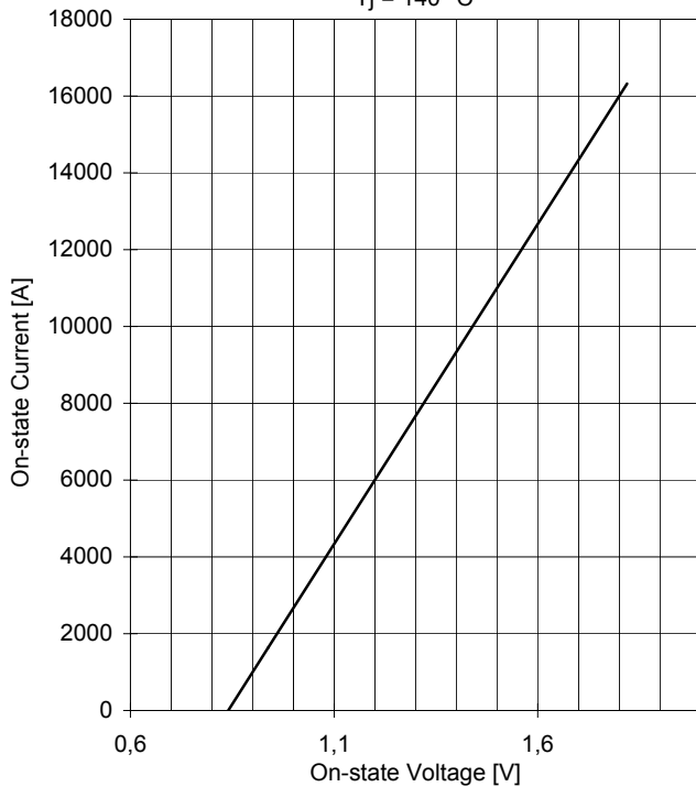
ON-STATE CHARACTERISTIC T_j = 140\text{ }^\circ\text{C}
