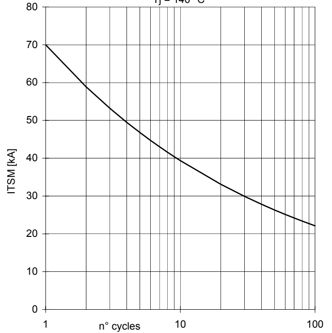
SURGE CHARACTERISTIC T_j = 140\text{ }^\circ\text{C}
