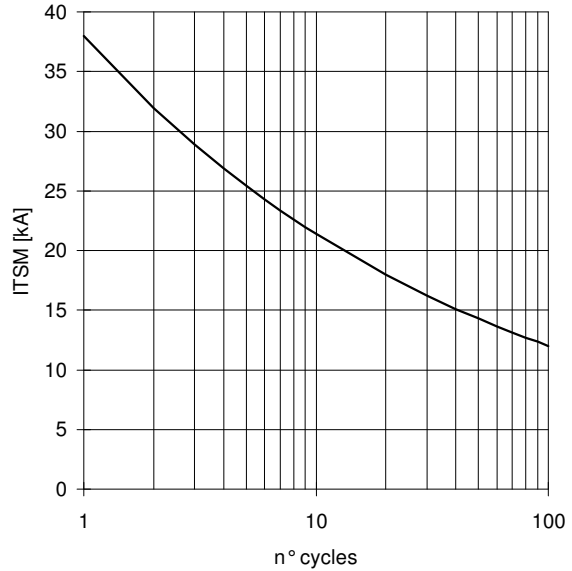
SURGE CHARACTERISTIC T j = 125 °C
