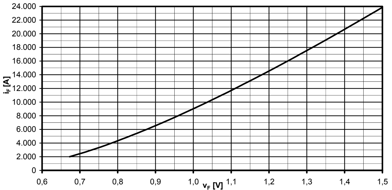
Grenzdurchlasskennlinie / Limiting on-state characteristic i_F = f(v_F)
