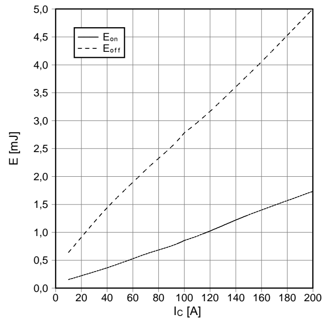
Schaltverluste IGBT-Wechselr. (typisch) switching losses IGBT-inverter (typical) E_{on} = f(I_c), E_{off} = f(I_c) V_{GE} = \pm 15\text{ V}, R_{Gon} = 2,2\ \Omega, R_{Goff} = 2,2\ \Omega, V_{CE} = 300\text{ V}, T_{vj} = 125^\circ\text{C}
