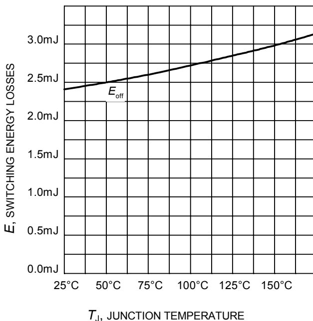
Figure 15. Typical turn-off energy as a function of junction temperature (inductive load, V_{CE}=600\text{V} , V_{GE}=0/15\text{V} , I_C=30\text{A} , R_G=28\Omega , Dynamic test circuit in Figure E)
