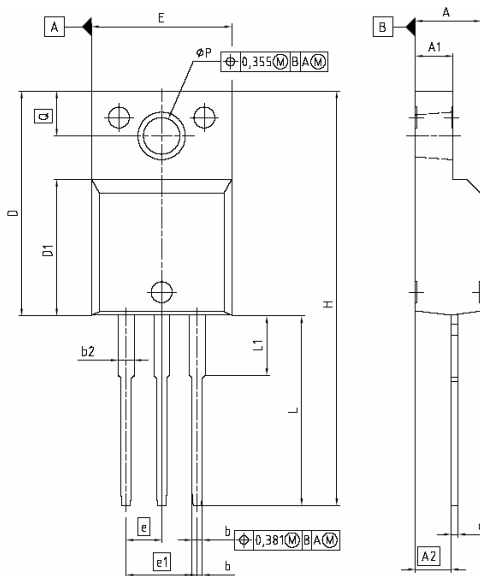
PG-TO220-3-31
