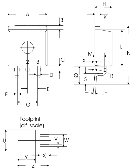
P-TO263-3-5
