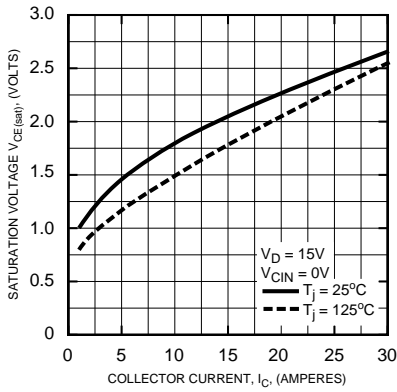
SATURATION VOLTAGE CHARACTERISTICS (TYPICAL)
