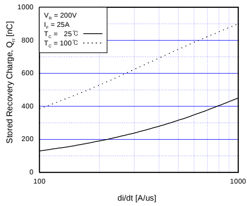
Fig 20. Stored Charge
