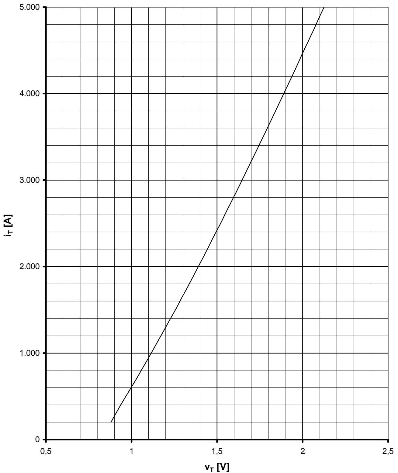
Grenzdurchlaßkennlinie / Limiting On-state characteristics i_T = f(v_T) T_{vj} = T_{vj} \text{ max}
