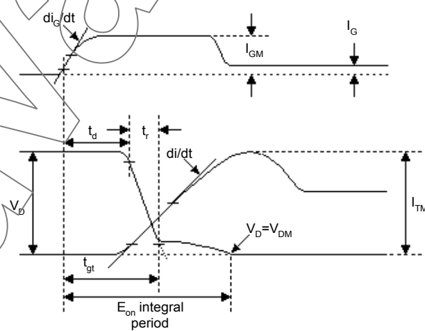
Diagram 9, Turn-on wave-diagrams.
